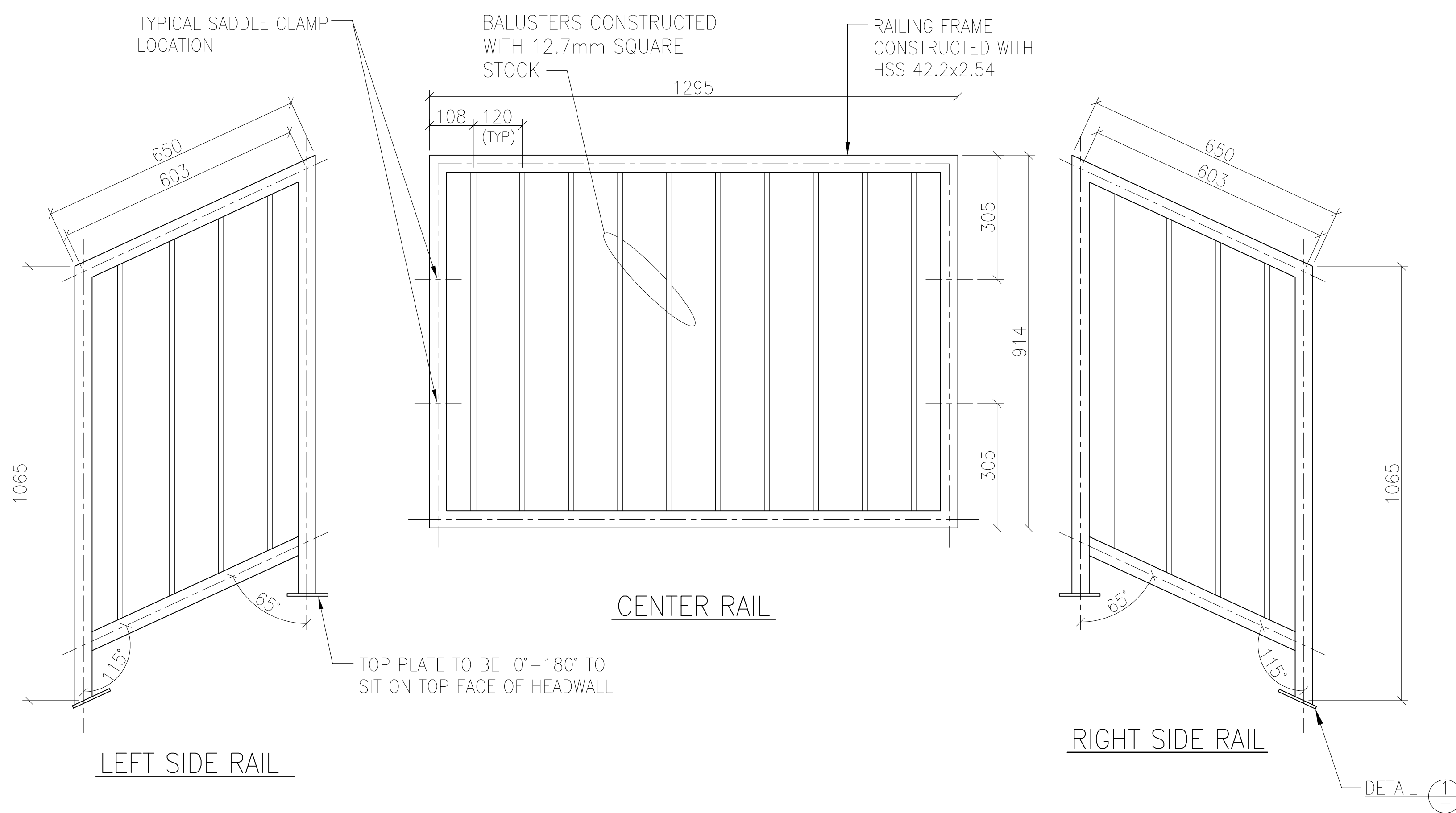
DEVELOPED ELEVATION
